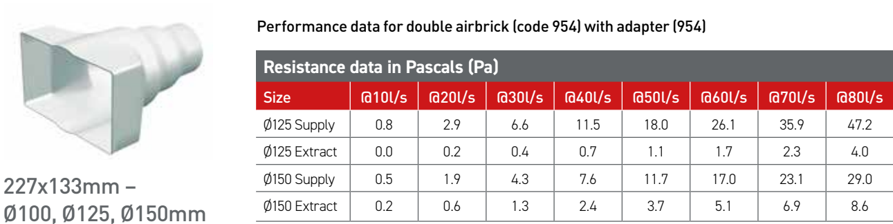
Performance data for Supply (air from outside)
