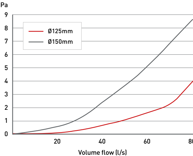
Performance data for Extract (air to outside)
